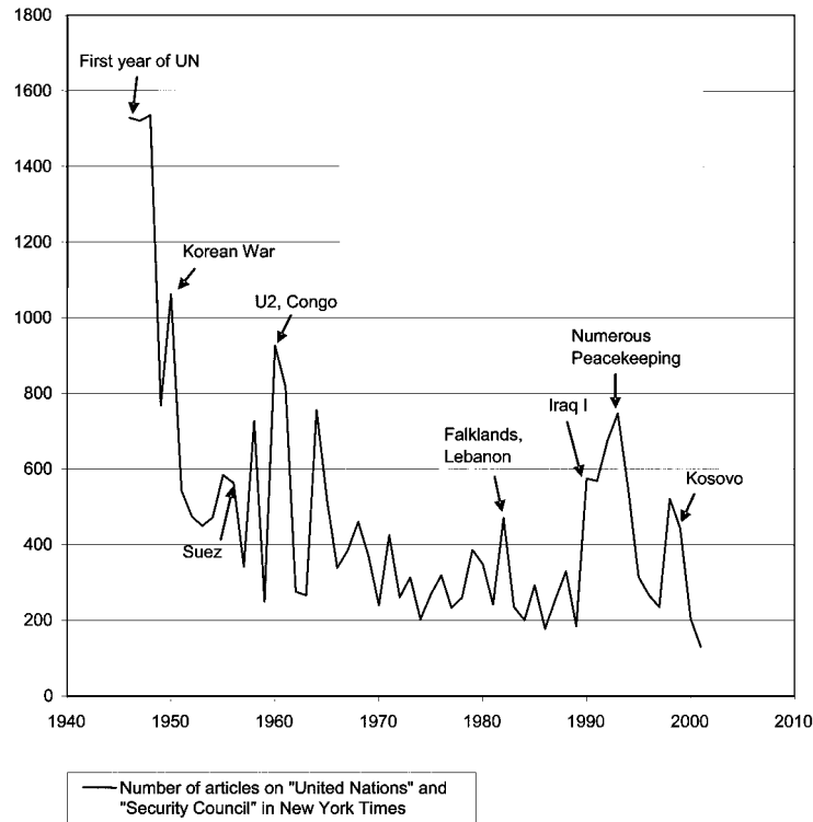
FIG. 1.—The New York Times variable
