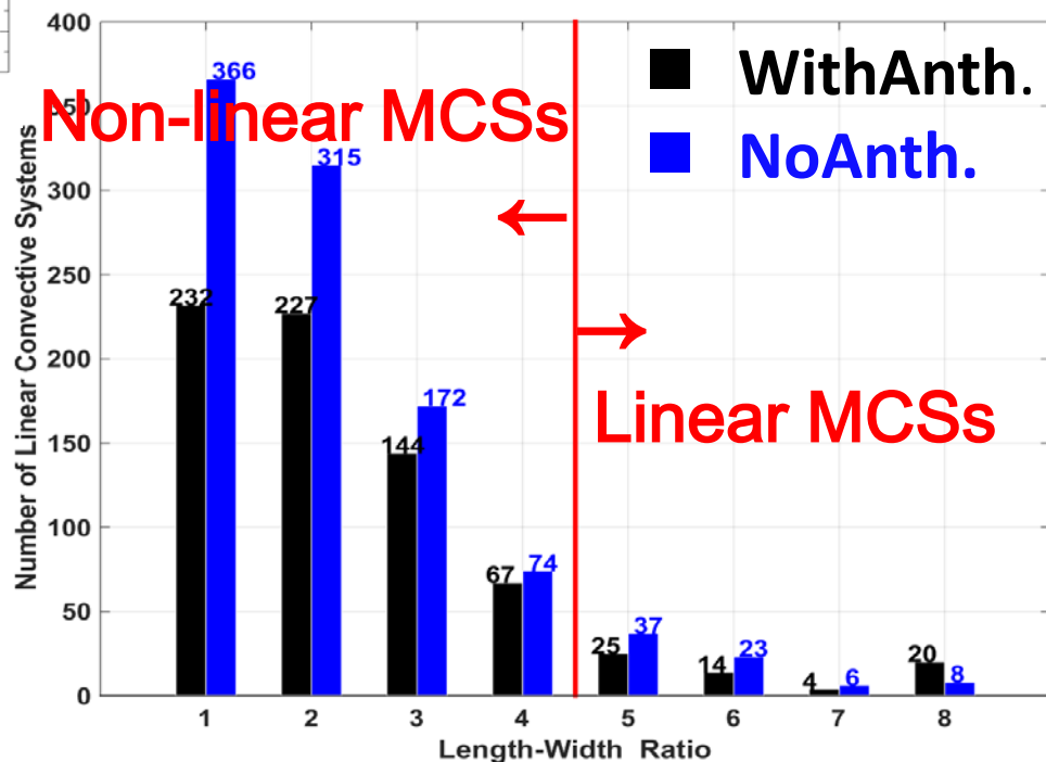
Number distribution of MCSs
