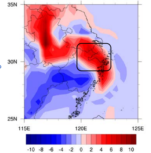
0827 reduction_O3_CTRL_YRD
