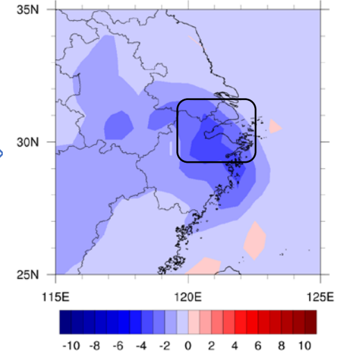
0827 reduction_O3_CTRLVOC_YRD
