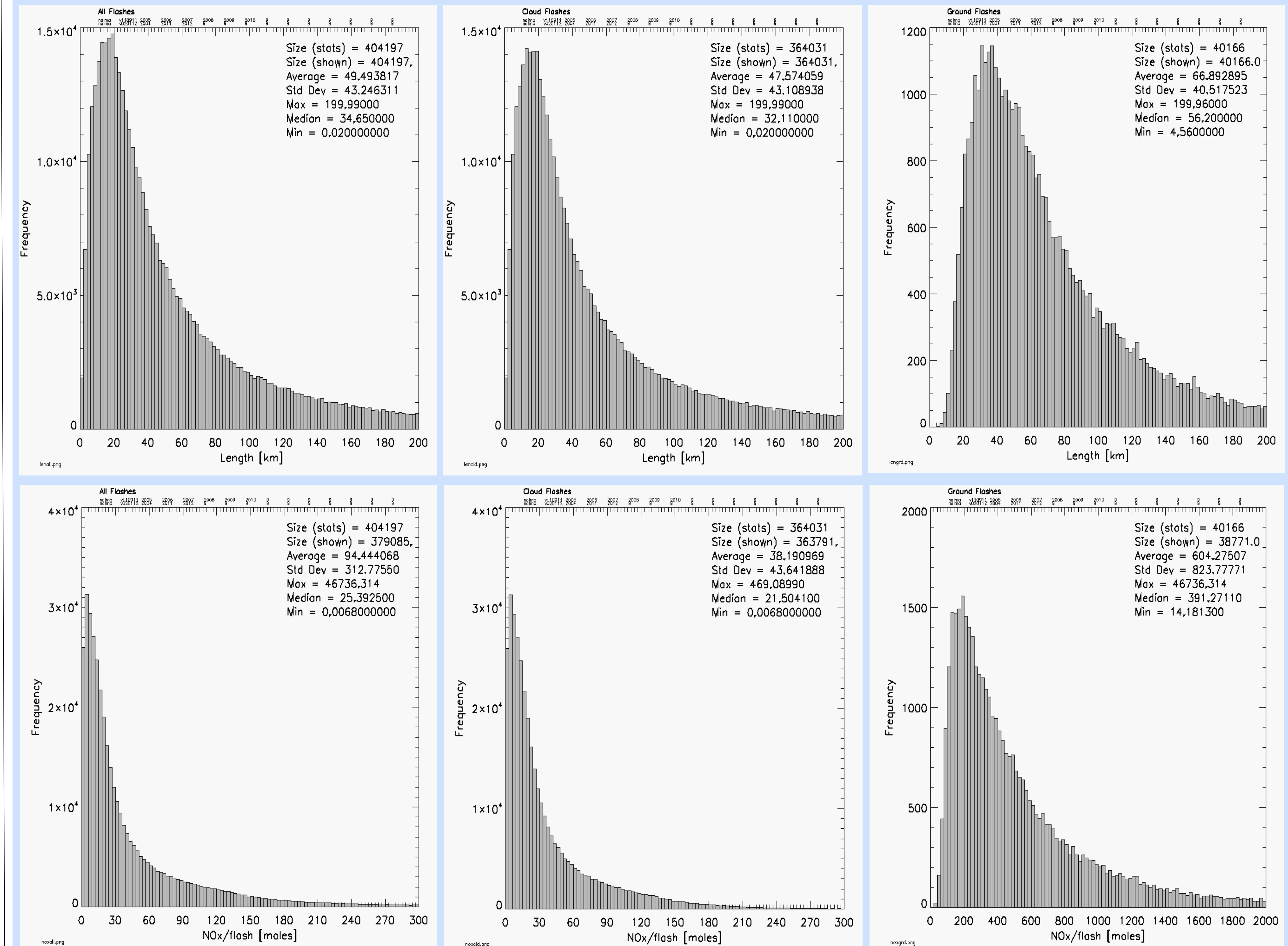
Figure 2. LNOM lightning channel length distributions (top 3 plots: all flashes, cloud flashes, ground flashes), and NOx per flash (bottom 3 plots). These distributions and associated statistics are derived from North Alabama thunderstorms.
