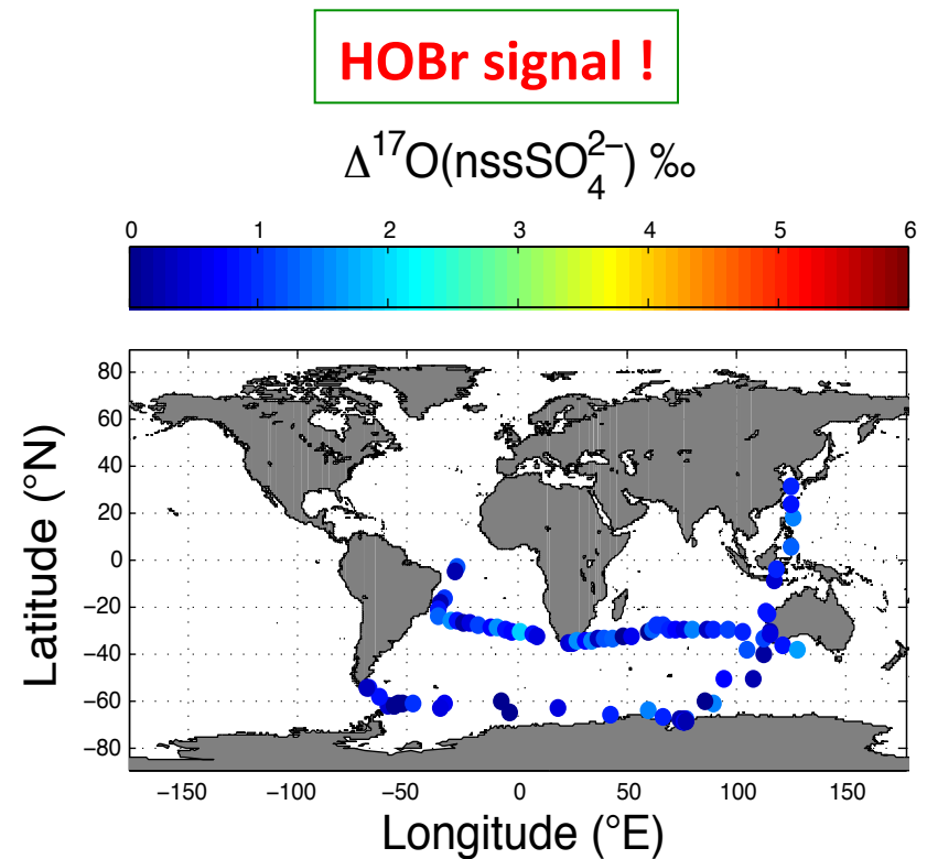
Fig. 2 Observational \Delta^{17}\text{O} of sulfate over the southern ocean.
