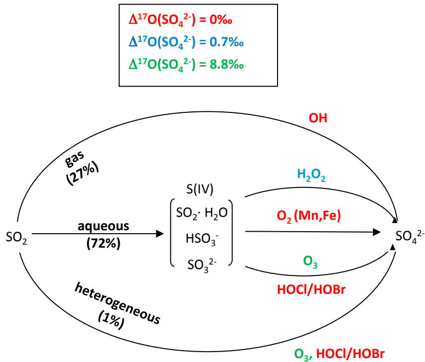
Fig. 1 Sulfate formation pathways and isotopic signatures.
