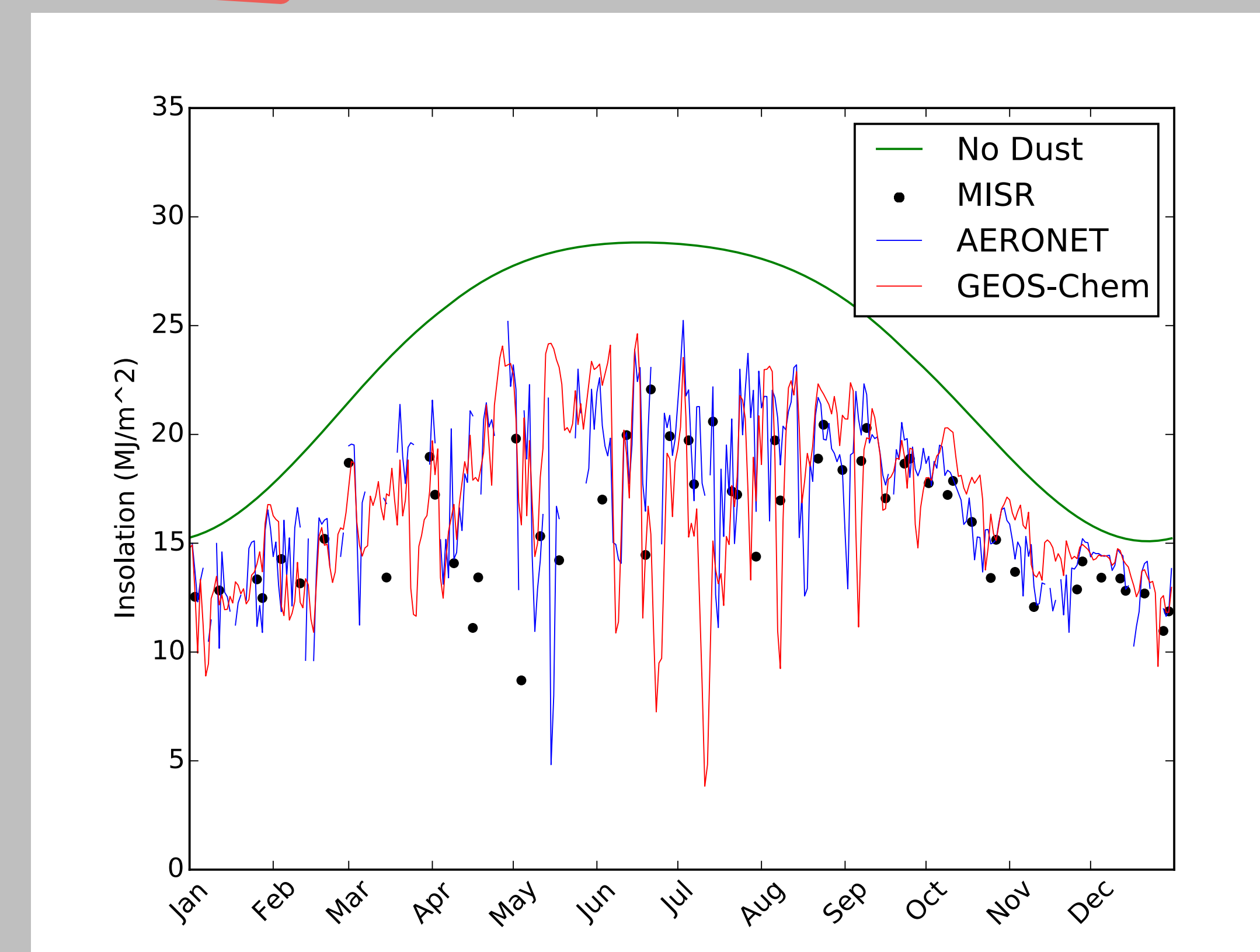
Diminished insolation's effect on PV Output
