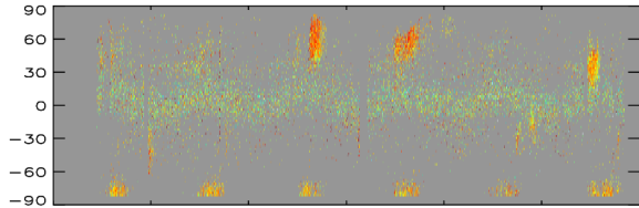
(b) Zonal mean of GEOS-Chem AOD (550 nm) over 10km
