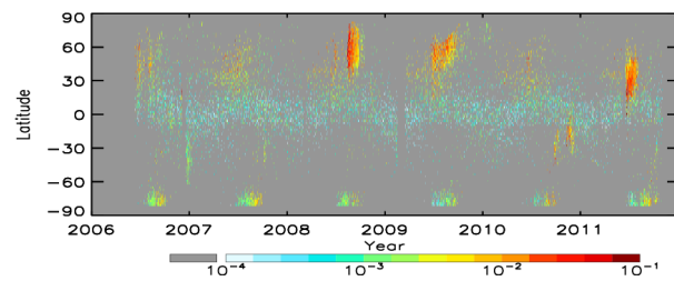
(b) Zonal mean of GEOS-Chem AOD (550 nm) over 10km
