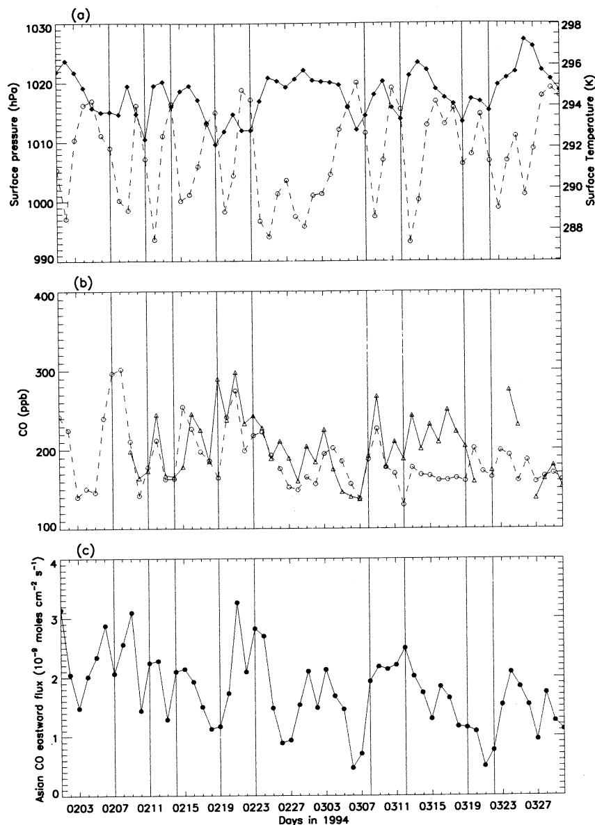
Figure 9. Time series of meteorological variables and CO concentrations for a site on the southern tip of Taiwan operated by Liu et al. [1997] in February-March 1994. (a) GEOS sea level surface pressure (solid line, left axis) and surface temperature (dashed line, right axis). (b) Observed CO concentrations (solid line) and corresponding model results (dashed line) obtained with the 2^\circ \times 2.5^\circ horizontal resolution version of the model. (c) Eastward fluxes of Asian CO ( 10^{-9} moles \text{cm}^{-2} \text{s}^{-1} ) through a wall located at 140^\circ\text{E} between 20^\circ and 40^\circ\text{N} . Vertical lines mark the passage of cold fronts at the site as reported by Liu et al. [1997].
