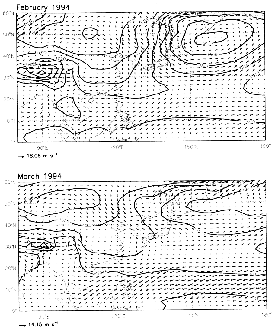
Figure 5. Monthly mean GEOS sea level pressures (hPa) for February and March 1994 and corresponding wind vectors at 250 m above the surface.
