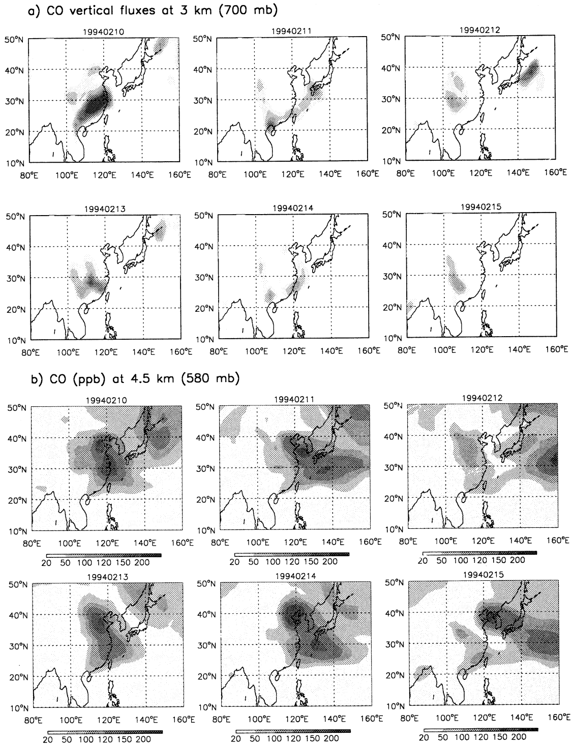
Figure 10. (a) Time series of CO vertical flux (moles \text{cm}^{-2} \text{s}^{-1} ) through the 3 km surface in the model. Shaded areas represent upward vertical CO fluxes. (b) Time series of CO concentrations (ppb) at 4.5 km altitude. Values are 24-hour average model results for individual days over the February 10–15, 1994 period.
