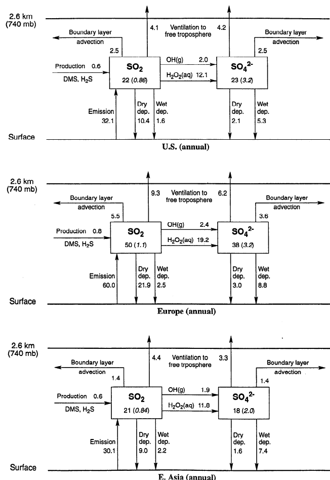
Figure 3. Annual mean regional budgets of SO 2 and SO 4 2- simulated by the model for the 0–2.6 km columns over the United States, Europe, and eastern Asia: inventories (Gg S), fluxes (Gg S d -1 ), and lifetimes for SO 2 and SO 4 2- (days, in parentheses). The horizontal extent of each region is shown in Figure 1. See caption to Figure 2 for definition of lifetimes.
