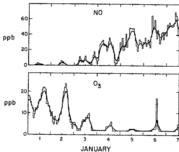
Fig. 6. Concentrations of NO and O 3 at Kernridge. The bold lines were obtained by smoothing the data with a digital filter.
