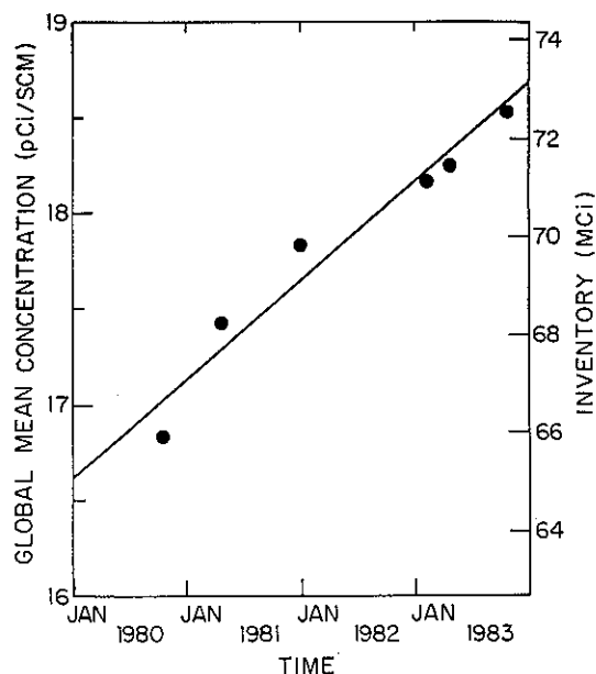
Fig. 2. Global inventory of ^{85}\text{Kr} derived from the model simulations. The line is a linear regression to the six points.
