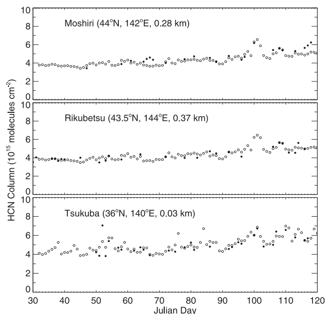
Figure 10. Time series of observed (solid circles) and simulated (open circles) 24-hour average HCN columns (molecules cm -2 ) at the three Japanese stations of Moshiri (44°N, 142°E, 0.28 km altitude), Rikubetsu (43.5°N, 144°E, 0.37 km altitude), and Tsukuba (36°N, 140°E, 0.03 km altitude) during TRACE-P (February–April 2001).
