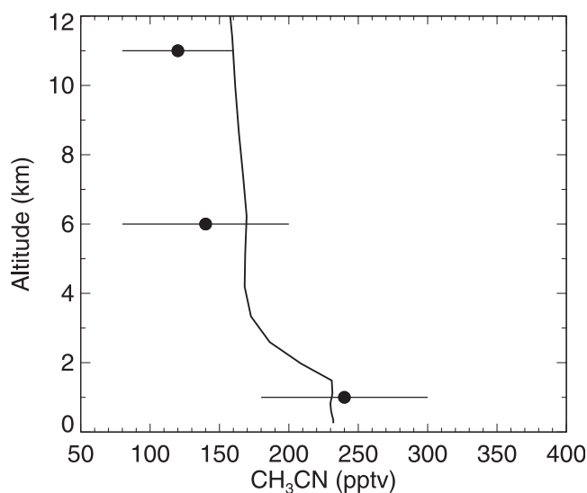
Figure 8. Vertical distribution of CH 3 CN concentrations over the northern Indian Ocean in March 2001. Median aircraft observations from the INDOEX campaign [de Laat et al. , 2001] are shown as symbols with standard deviations. Monthly mean model results for the corresponding month and region (0–10°N, 65°E–80°E) are shown as the solid line.
