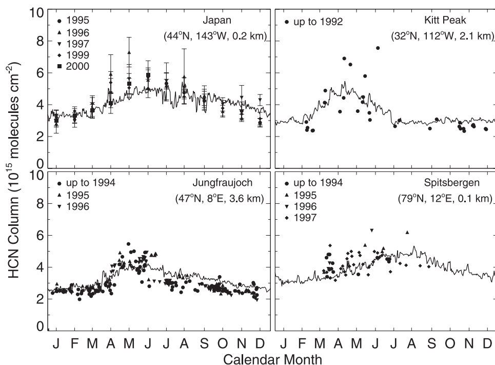
Figure 12. Monthly mean HCN total columns ( \text{molecules cm}^{-2} ) retrieved from spectroscopic measurements at Moshiri and Rikubetsu in Japan [Zhao et al. , 2000, 2002], Kitt Peak in Arizona [Mahieu et al. , 1995], Jungfraujoch in the Swiss Alps [Mahieu et al. , 1995, 1997], and Ny Ålesund in Spitsbergen [Li et al. , 2000]. Data for the two Japanese sites are monthly means and vertical bars indicate standard deviations. The solid lines represent simulated daily average HCN total columns for 2000.
