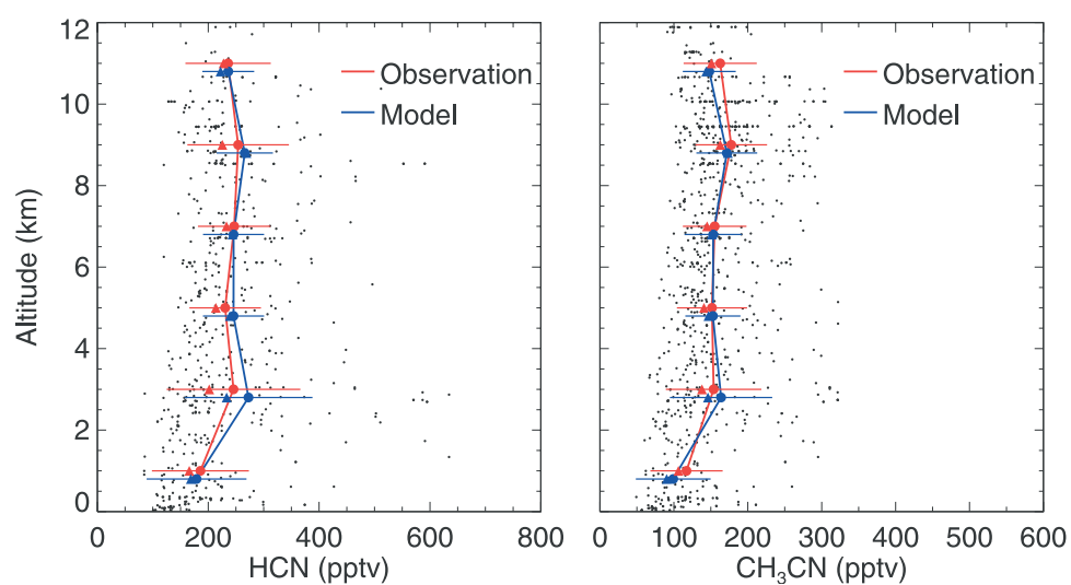
Figure 2. Vertical distributions of HCN and CH 3 CN observed in TRACE-P over the North Pacific under background conditions ( \text{CO} < 120 ppbv and \text{C}_2\text{Cl}_4 < 10 pptv). Individual observations are shown as dots. Solid circles, triangles, and horizontal bars represent means, medians, and standard deviations, respectively.
