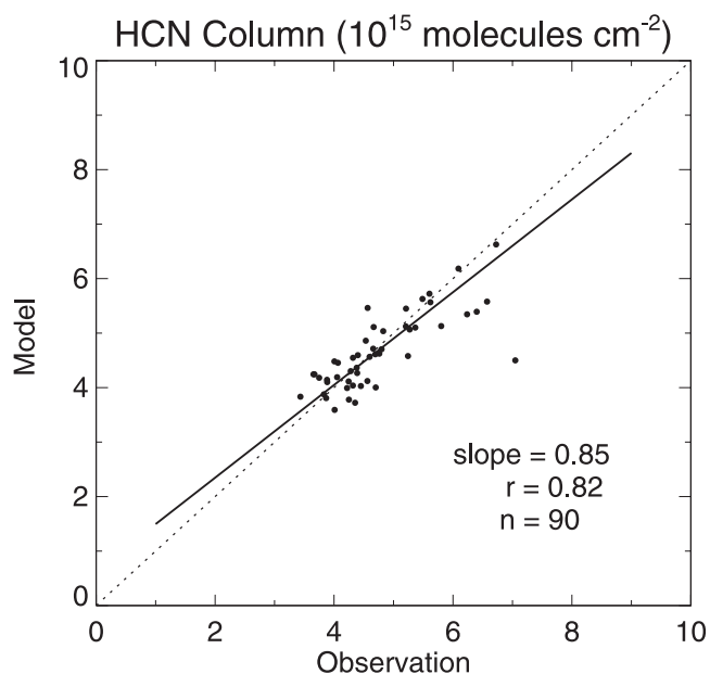
Figure 11. Scatterplot of observed and simulated daily HCN columns ( \text{molecules cm}^{-2} ) at the Moshiri, Rikubetsu, and Tsukuba Japanese sites during TRACE-P. Values are averages over the three sites. The regression line is calculated without the outlier.
