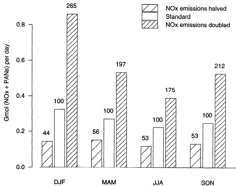
Figure 12. Seasonal mean export fluxes of \text{NO}_x + \text{PANs} from the U.S. boundary layer in the standard simulation and in simulations with halved or doubled \text{NO}_x emissions. The percentage changes in the export fluxes for each season, relative to the standard simulation (100%), are shown on top of the bars.
