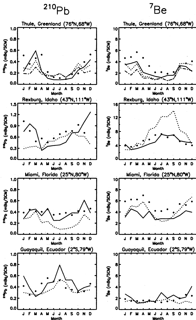
Figure 8. Comparison between observed (solid line) and simulated (dotted line) seasonal variations of ^{210}\text{Pb} and ^7\text{Be} concentrations at the sites of Thule (1994), Rexburg (1993), Miami (1991), Guayaquil (1992), Tutuila (1994), Santiago (1992), and South Pole Station (1991). The model simulation uses meteorological data for the appropriate year. Also shown as dots are the long-term climatologies of observations at the sites for ^{210}\text{Pb} (K96) and ^7\text{Be} [Feely et al. , 1989]. The dot-dashed lines for Thule and South Pole Station indicate the model results for a simulation where in-cloud scavenging below 258 K is not suppressed (the effect at other sites is negligibly small).
