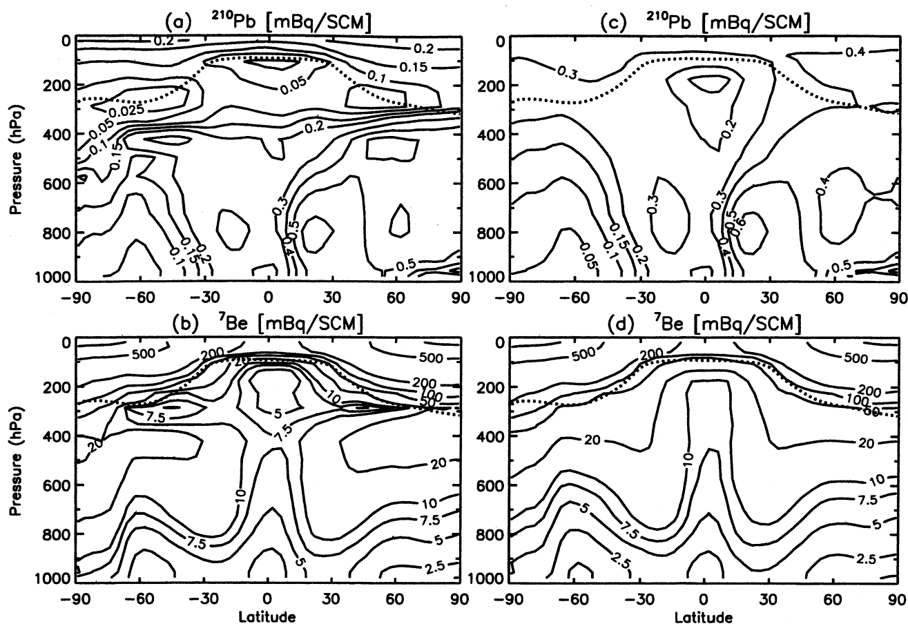
Figure 3. Zonal mean mixing ratios ( \text{mBq SCM}^{-1} ) of (a) ^{210}\text{Pb} and (b) ^7\text{Be} in the standard simulation as a function of latitude and pressure. (c, d) Same as Figures 3a and 3b, except that aerosol scavenging by cirrus precipitation is excluded. Values are annual averages for 1994. For the simulation of ^7\text{Be} in the troposphere the ^7\text{Be} source in the stratosphere (diagnosed from the local model tropopause) has been reduced by a factor of 4 to correct for excessive cross-tropopause transport in the model (section 2.6); this reduction is not applied to the simulation of ^7\text{Be} in the stratosphere. The dotted line is the annual average tropopause height.
