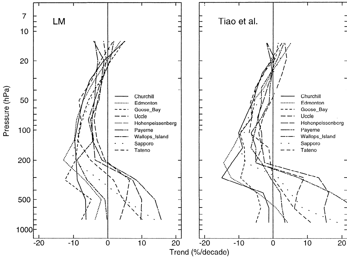
Figure 9. Annual trends for individual sonde stations located between 36° and 59°N, superimposed. Updated from WMO [1998].
