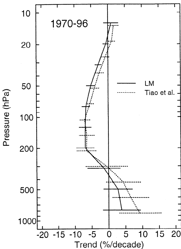
Figure 10. Mean annual trend for the sonde stations located between 36° and 59°N. The solid line shows the LM results; the dashed line shows the Tiao et al. results. Two standard errors are shown; these were calculated as the usual standard error for the sample mean of the nine annual estimates (one third of the standard deviation of the nine trend estimates), for each pressure level. Updated from WMO [1998].
