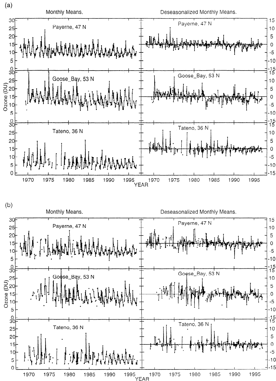
Figure 3. Time series of monthly mean values for ozone in DU and deseasonalized monthly means for selected stations. (a) The correction factors used by LM were applied, and (b) the data selection criteria used by Tiao et al. were applied (see text). Values are shown for one of the 33 levels near 90 hPa, and the same relative scale is used for both sets of means. Adapted from WMO [1998].
