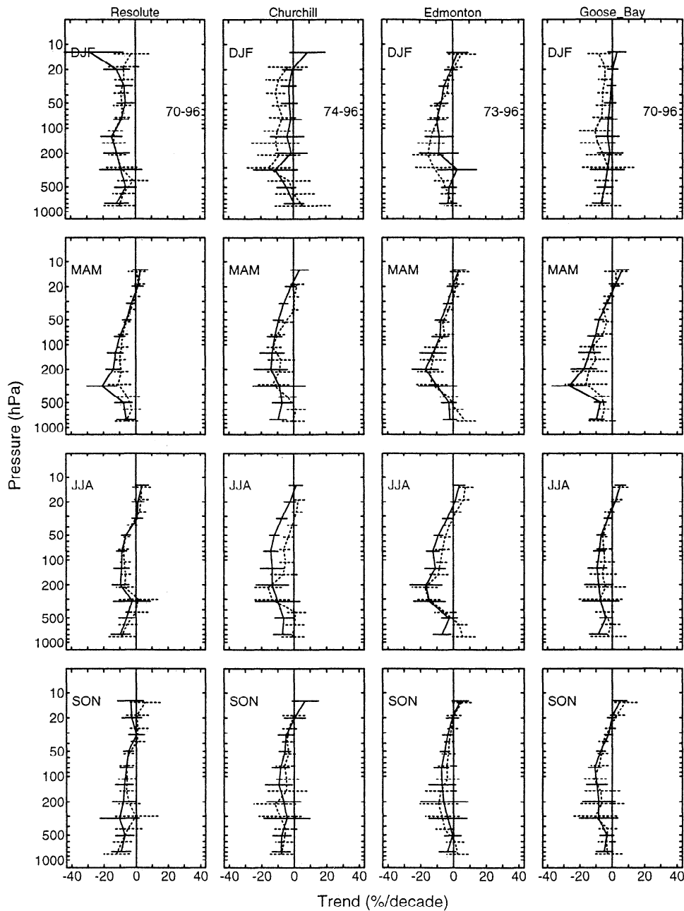
Figure 5. Seasonal trends in the vertical distribution of ozone for 1970-1996. The results of LM are shown by the solid line, and the Tiao et al. results are shown by the dotted line. Two standard errors are shown. Trends are plotted at the midpoint of the pressure levels used in each analysis. Updated from WMO [1998].
