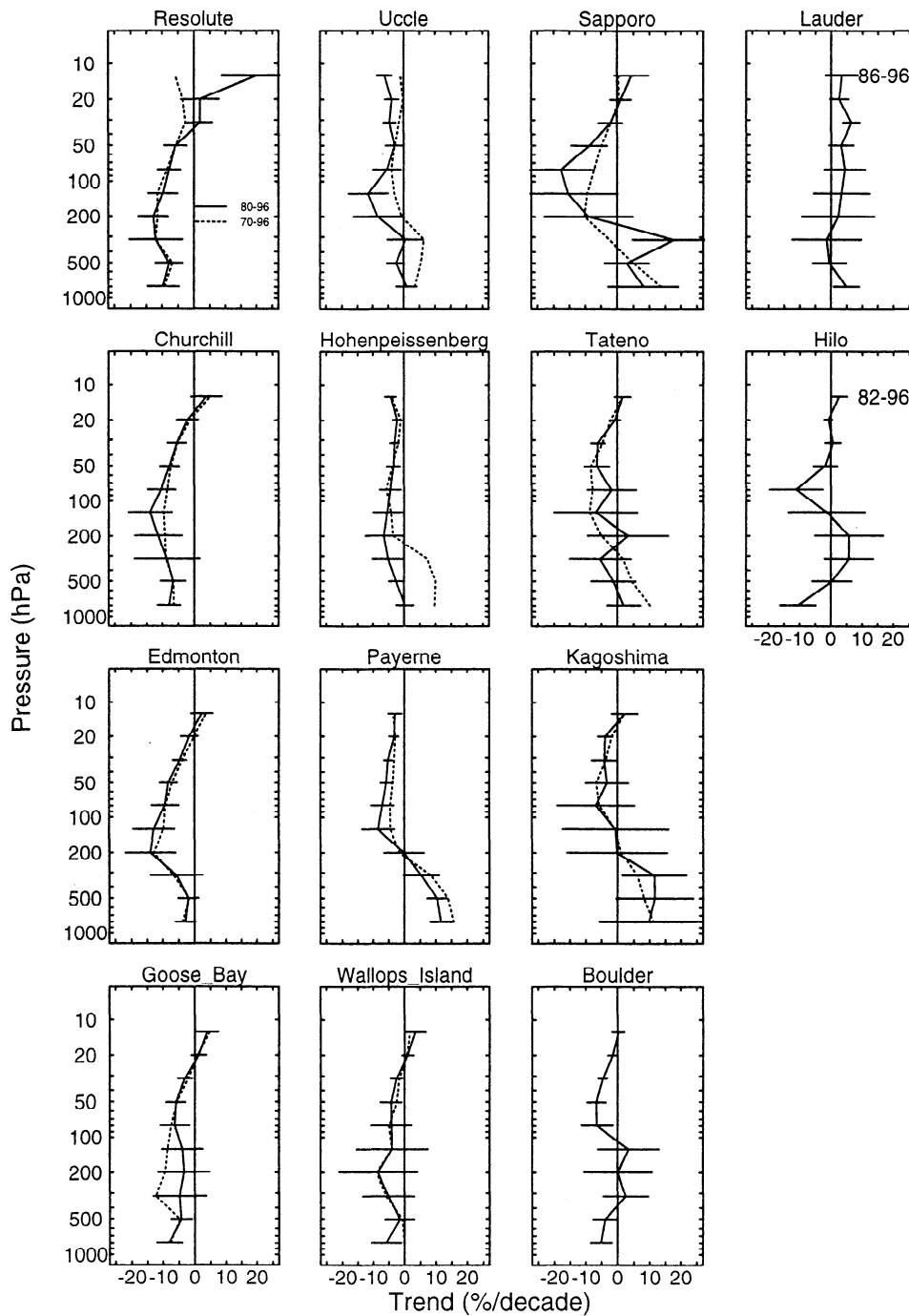
Figure 14. Annual trends for 1980-1996 (solid lines) compared to trends for 1970-1996 (dashed lines) where available. The Lauder trends are for 1986-1996, and the Hilo trends are for 1982-1996. LM results are shown. Updated from WMO [1998].
