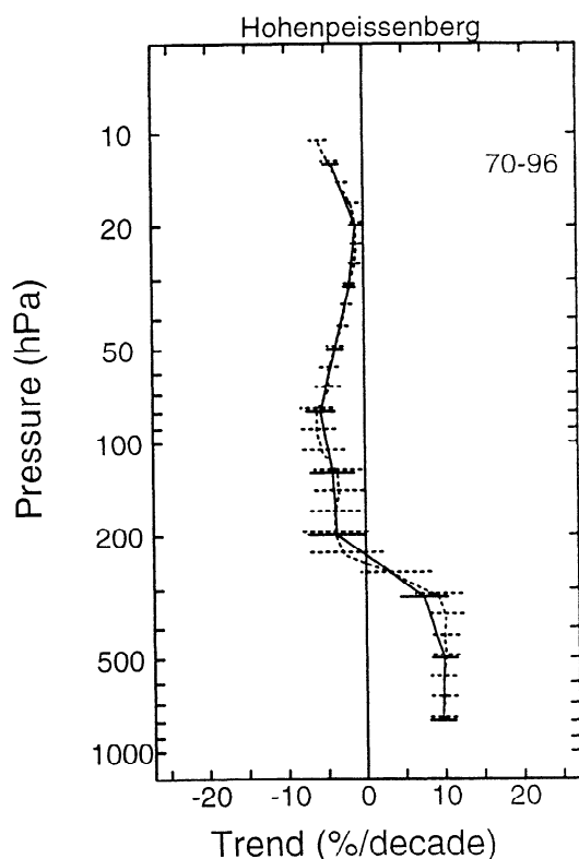
Figure 2. Annual trends in the vertical distribution of ozone for 1970-1996 for Hohenpeissenberg, in percent per decade. The dashed line shows trends computed by LM for the ozone column in 33 layers equally spaced in log pressure from 1000 to 6.3 hPa. The solid line shows results for 11 layers obtained by summing the ozone content in 3 consecutive layers. Results are shown below 10 hPa.
