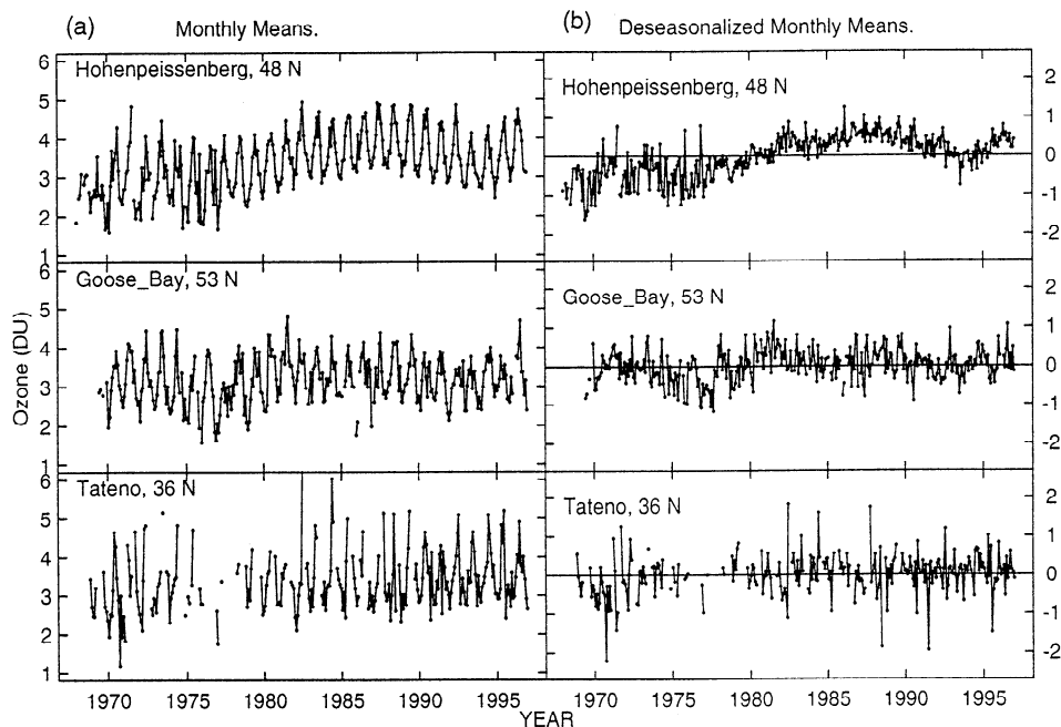
Figure 16. Time series of (a) monthly mean values for ozone in DU and (b) deseasonalized monthly means for selected stations. The correction factors used by LM were applied (see text). Values are shown for one of the 33 levels near 500 hPa, and the same relative scale is used for both sets of means. From WMO [1998].
