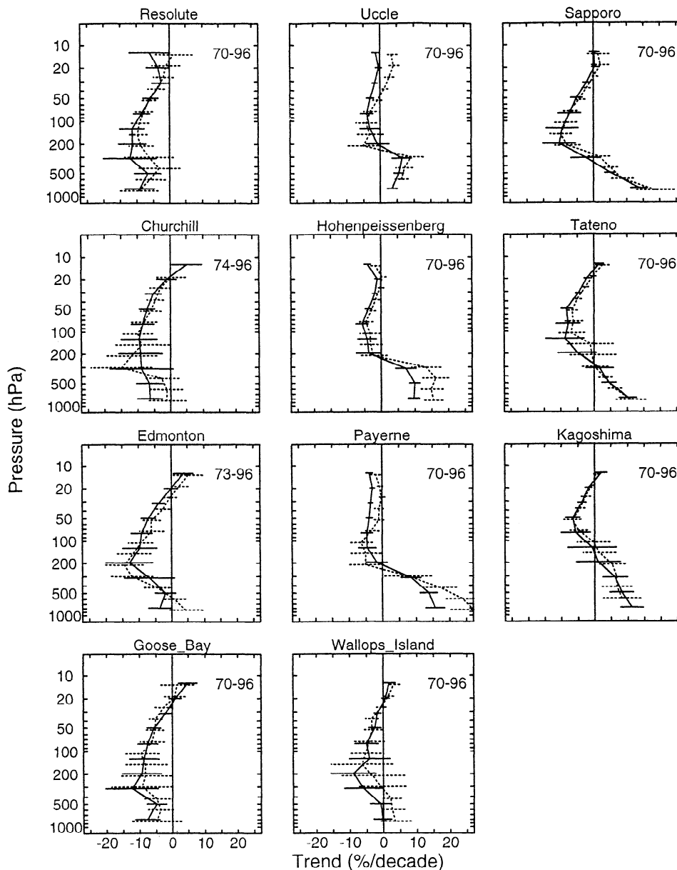
Figure 6a. Annual trends in the vertical distribution of ozone for 1970-1996. The results of LM are shown by the solid line and the Tiao et al. results are shown by the dotted line. Two standard errors are shown. Updated from WMO [1998].
