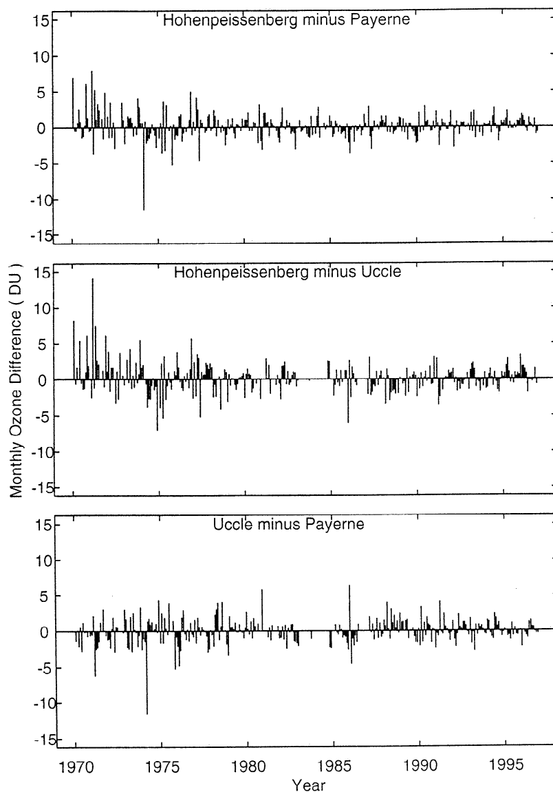
Figure 4. Difference of monthly mean values for the three European stations near 90 hPa. The correction factors used by LM were applied (see text). Adapted from WMO [1998].
