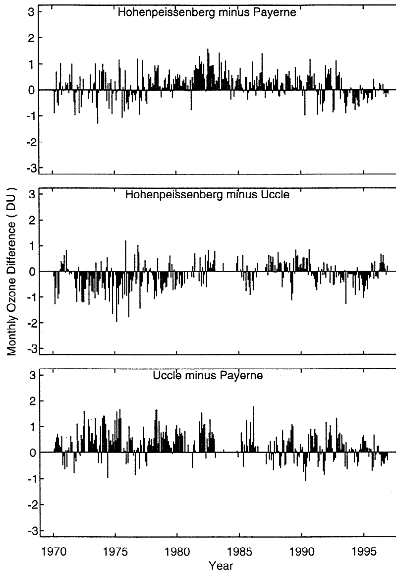
Figure 17. Difference of monthly mean values for the three European stations near 500 hPa. The correction factors used by LM were applied (see text). From WMO [1998].
