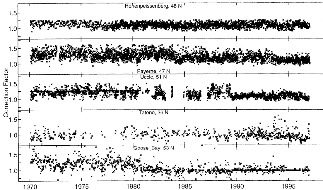
Figure 1. Correction factors for selected sonde stations. Adapted from WMO [1998].
