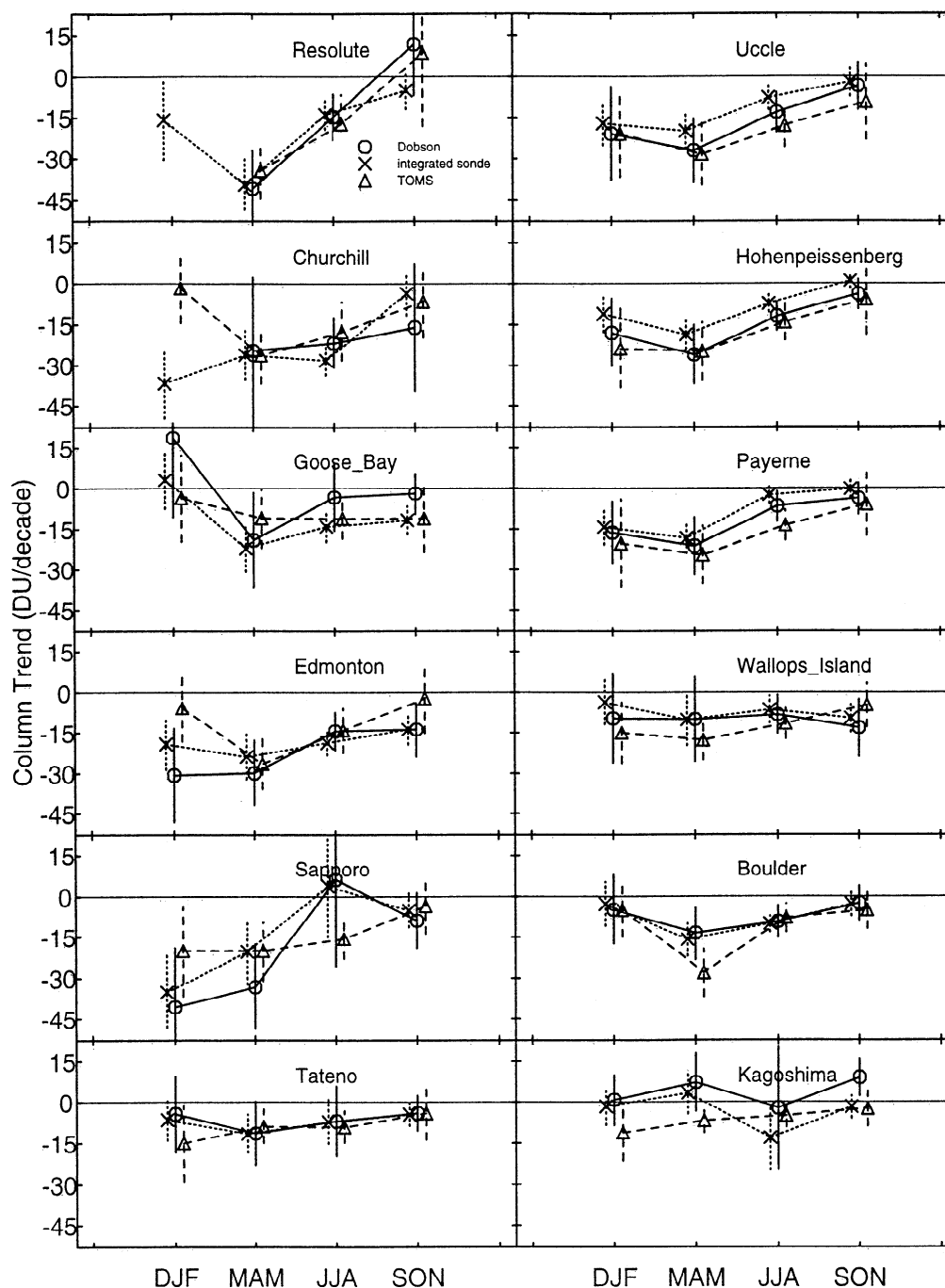
Figure 20. Comparison of column trends for ozone for 1980-1996. Circles and crosses show the column and integrated sonde trends defined as in Figure 19. The sonde results are the LM analysis. The triangles show the trend in TOMS data from November 1978 to October 1994, computed by Hollandsworth. The three results for each season are offset for clarity. Updated from WMO [1998].
