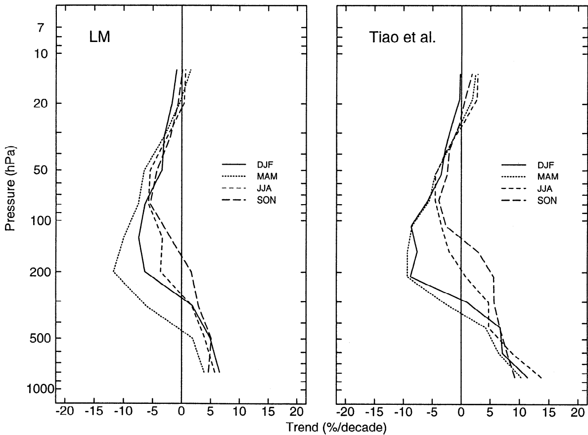
Figure 13. Seasonal mean profiles for stations located between 36° and 53°N. (a) LM results, and (b) Tiao et al. results are shown. Updated from WMO [1998].
