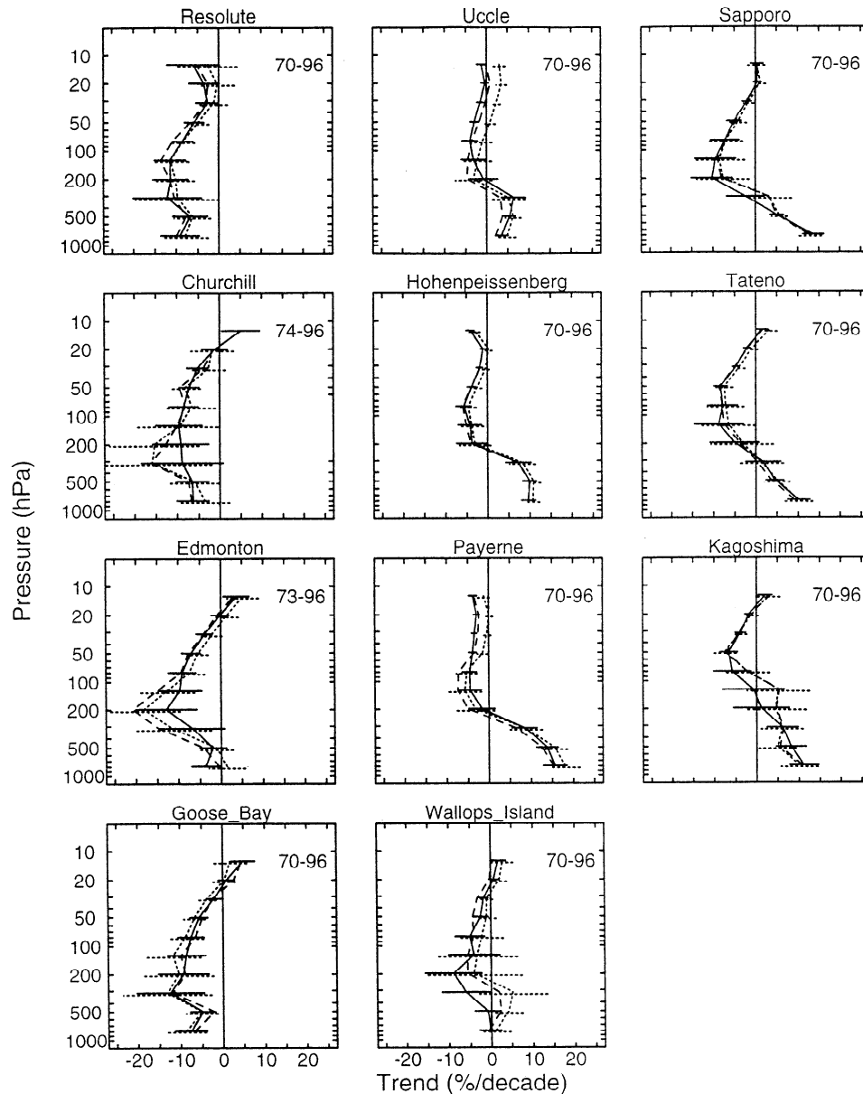
Figure 7. Sensitivity of annual trends in the vertical distribution of ozone to data treatment prior to trend analysis. All trends were derived with the LM model. The solid line shows results for the LM data selection criteria; the dotted line shows results with the Tiao et al. data selection criteria and with the data divided by the CF; the dashed line shows results with the Tiao et al. data selection criteria but without dividing by the CF. Updated from WMO [1998].
