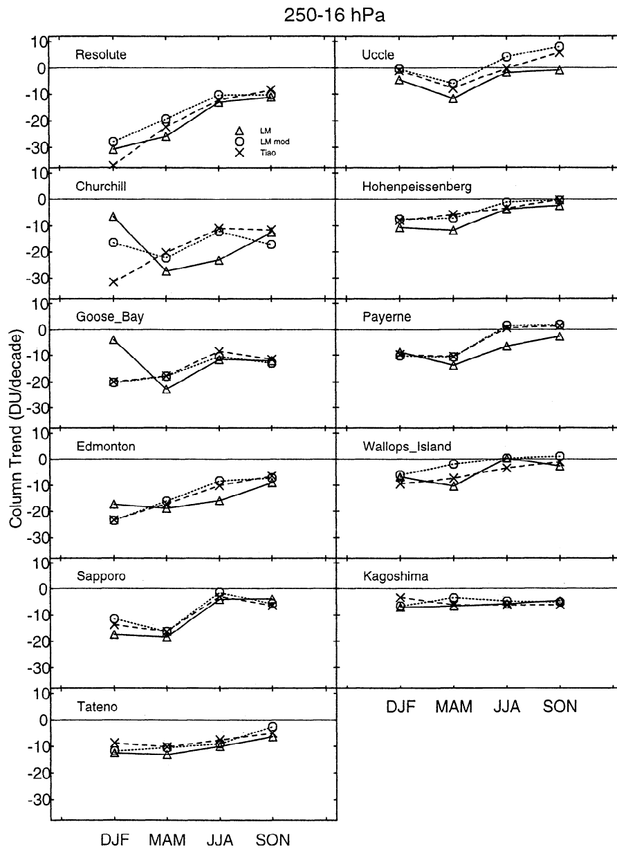
Figure 8. Column trend in ozone in DU/decade from 250 to 16 hPa for 1970-1996. The triangles are results from LM, the crosses are those from Tiao et al., and the circles are results for the LM model, with the data treatment of Tiao et al. (their data selection and with the data divided by the CF). Updated from WMO [1998].
