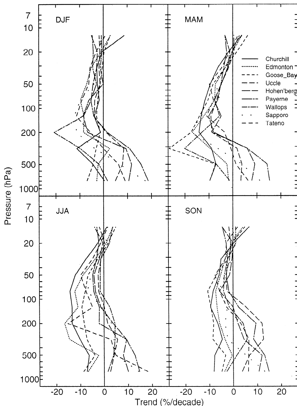
Figure 11. Seasonal mean trends for the sonde stations located between 36^{\circ} and 59^{\circ} N, superimposed. LM results are shown. Updated from WMO [1998].
