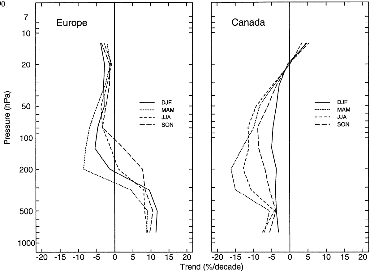
Figure 12. Seasonal mean profiles for (a) three European stations, 48°-51°N and for (b) three Canadian stations, 53°-59°N. LM results are shown. Updated from WMO [1998].
