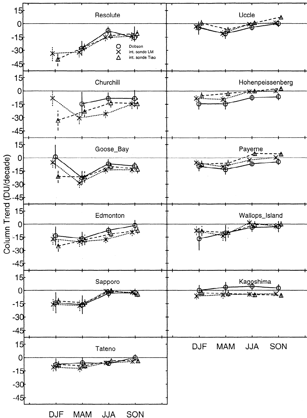
Figure 19. Comparison of column trends for ozone for 1970-1996. The circles show the trend in the overhead ozone column measured on the same days as the sondes used in the LM analysis, computed with the LM model. The crosses show the integrated sonde trend up to 16 hPa, computed with the LM model, and the triangles show the integrated sonde trend up to 16 hPa computed with the Tiao et al. model. Two standard errors are shown. The errors for the sonde data are only approximate, as they do not account for any correlation between ozone at one layer and the next, and the Tiao et al. errors are smaller because they are for 12 layers rather than 9. The three results for each season are offset for clarity. Updated from WMO [1998].
