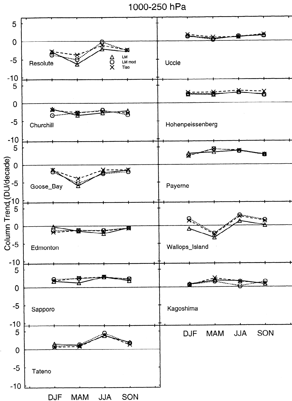
Figure 18. Column trend in ozone in DU/decade from the lowest layer to 250 hPa. The triangles are results from LM, the crosses are those from Tiao et al., and the circles are results for the LM model, with the data treatment of Tiao et al. (their data selection and with the data divided by the CF). Updated from WMO [1998].
