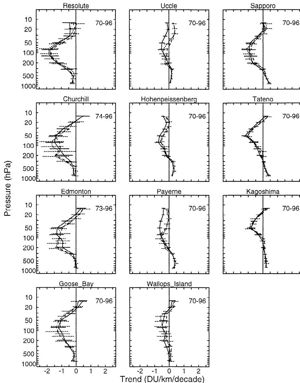
Figure 6b. Annual trends in the vertical distribution of ozone for 1970-1996 in DU/km/decade. Pressure was converted to altitude using the U.S. Standard Atmosphere. The results of LM are shown by the solid line, and the Tiao et al. results are shown by the dotted line. Two standard errors are shown. The dashed line shows trends derived with the LM model run with the Tiao et al. data treatment (their selection criteria and with the data divided by the CF). Updated from WMO [1998].
