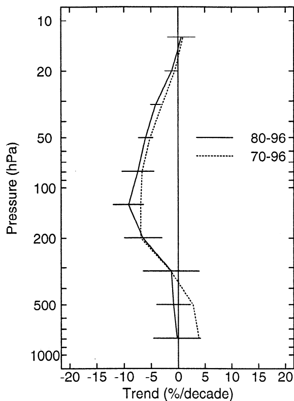
Figure 15. Mean annual trend for the sonde stations located between 36^{\circ} and 59^{\circ} N (excluding Boulder), for 1980-1996 (solid line) compared to the mean trend for 1970-1996 (dotted line). LM results are shown. Two standard errors are shown, calculated as in Figure 10. Updated from WMO [1998].
