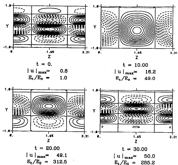
FIG. 7. Development of the perturbation streamwise velocity u at x=0 for the perturbation with maximum energy growth at \tau=20 in Couette flow with R=1000 , located at \alpha=0.46 , \beta=1.9 . Values are normalized by the maximum value of v at time t=0 .
