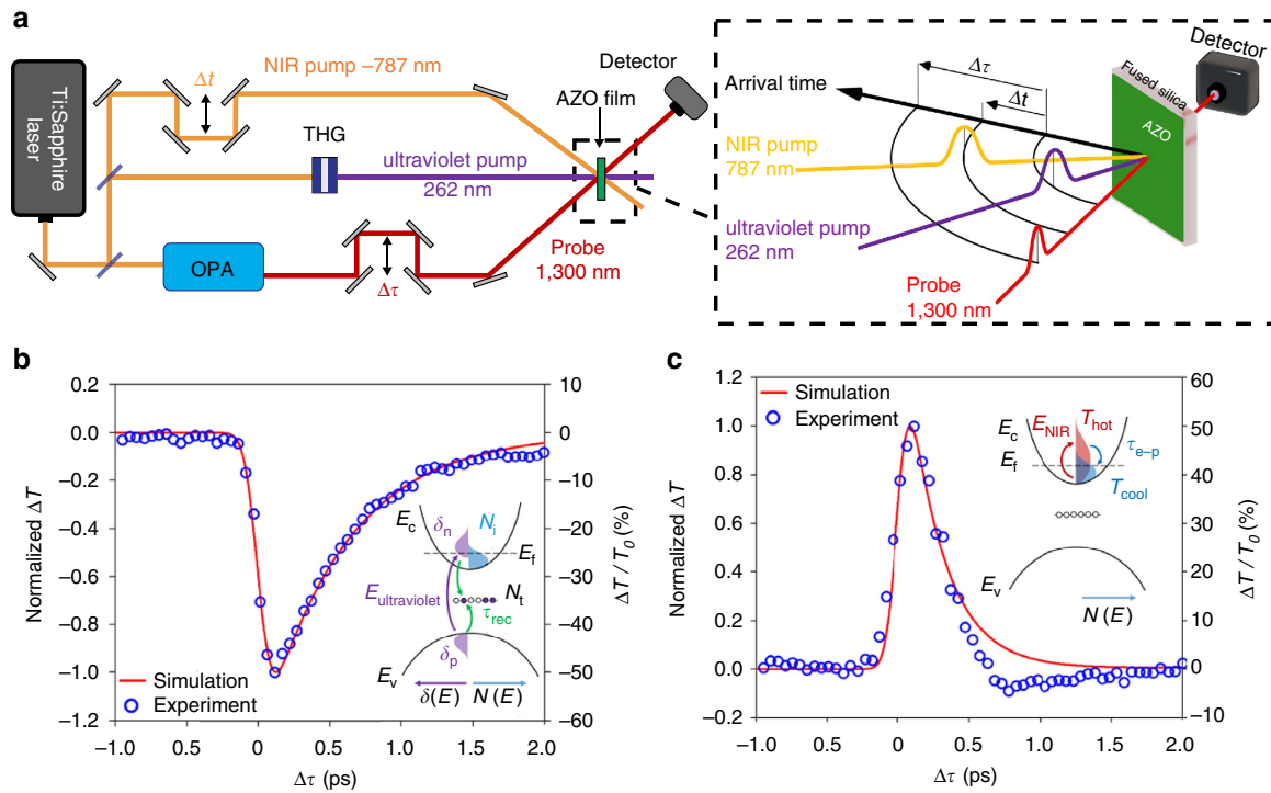
Figure 1 | Two-colour pump-probe experiment. (a) Schematic of the two-colour pump-probe experimental set-up where the two pump wavelengths, 787 nm (NIR) and 262 nm (ultraviolet), are illustrated along with the probe wavelength of 1,300 nm. The delay between the two pump pulses is denoted \Delta t while the delay between the probe and ultraviolet signal is denoted \Delta \tau . For intraband excitation using only the NIR pump, \Delta \tau is defined as the delay between the probe and NIR pump pulse arrival time. The black arcs indicate the arrival time of the pulses. (b) Change in transmission at 1,300 nm versus the pump-probe delay \Delta \tau under 262 nm excitation fitted with simulation. The inset illustrates the process diagram for interband excitation: ultraviolet light ( E_{\text{ultraviolet}} ) generates electron-hole pairs ( \delta_n, \delta_p ) above the Fermi level ( E_f ) in addition to the intrinsic concentration ( N_i ), which recombine through mid-gap trap states ( N_t, \tau_{\text{rec}} ). (c) Change in transmission at 1,300 nm versus the pump-probe delay \Delta \tau under 787 nm excitation fitted with simulation. The inset illustrates the process diagram for intraband excitation: NIR light ( E_{\text{NIR}} ) raises the temperature of conduction band electrons ( T_{\text{cool}} \rightarrow T_{\text{hot}} ), which relax through scattering processes ( \tau_{e-p} ), heating the lattice. The change in transmission from the experiment was obtained through \Delta T = (T - T_0)/T_0 , where T_0 is the transmission of the probe far from the pump pulse. For comparison with the theoretical results, the amplitude of the induced transmission change was normalized using \Delta T_{\text{normalized}} = \Delta T/|\Delta T_{\text{max}}| , where |\Delta T_{\text{max}}| is the magnitude of the peak change in transmission. The same procedure was completed for the simulation results.
