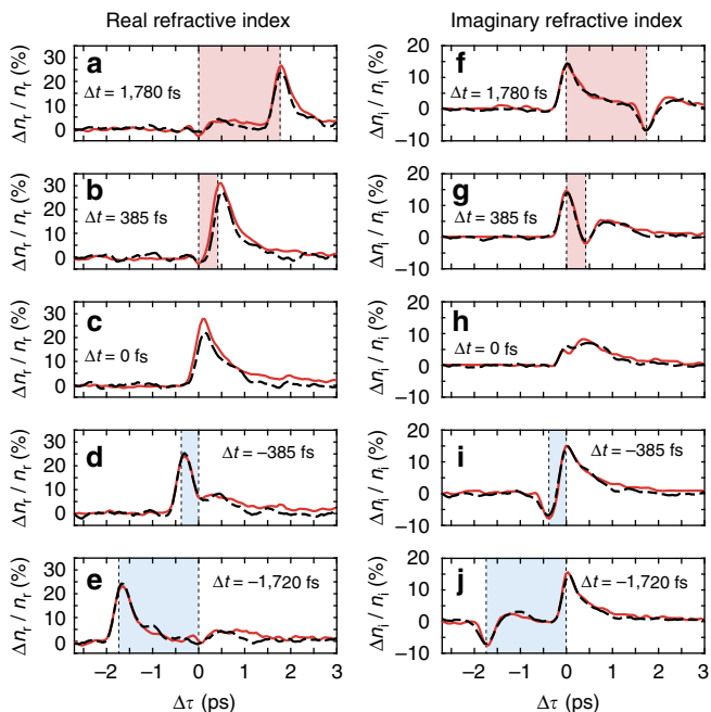
Figure 2 | Dynamic change in the optical response of AZO thin films triggered by two-colour excitation. Percentage change of the real (a–e) and imaginary (f–j) part of the refractive index as a function of the delay \Delta\tau between the ultraviolet pump and the infrared probe pulses. Multiple vertical plots are shown, for different delay \Delta t between the ultraviolet and the NIR pump pulses. Shaded areas indicate whether the ultraviolet pump, which is used as time reference, precedes (light blue) or follows (light red) the NIR pump. Overlapping the results obtained by simultaneous two-colour pumping (red curves), we plot the computed change in refractive index calculated by the algebraic summation of the results obtained from experiments with separate ultraviolet and NIR pump pulses (black dashed curves). The probe, the NIR and the ultraviolet pump wavelengths were set to 1,300 nm, 787 nm and 262 nm, respectively. The probe intensity was low: I_p \approx 200 \text{ MW cm}^{-2} , while the pump fluences were F_{\text{ultraviolet}} = 5 \text{ mJ cm}^{-2} and F_{\text{NIR}} = 14 \text{ mJ cm}^{-2} .
