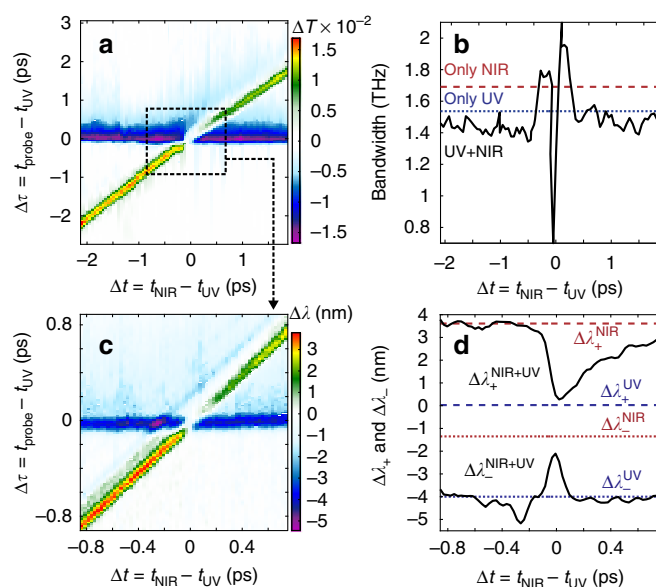
Figure 3 | Two-colour pumping effects. (a) Change in the probe pulse transmission as a function of the pump-probe delay ( \Delta\tau ) and the inter-pump delay ( \Delta t ). The ultraviolet (UV) pump decreases the transmission, whereas the NIR increases it. The combined effect produces a \Delta t -dependent modulation. The modulation bandwidth is evaluated by performing a Fourier transform along \Delta\tau , and is shown by the black curve in (b). For delays close to \Delta t = 0 , the modulation bandwidth can be decreased or increased by the two-colour combined effect. The blue and red dashed lines show the bandwidth of the ultraviolet-only and NIR-only driven modulation. (c) Measured central wavelength shift of the transmitted probe pulse ( \approx 15 \text{ nm} bandwidth) in a zoomed \Delta t - \Delta\tau region (square box in (a)). The ultraviolet pump blue shifts the probe wavelength, whereas the NIR pump does the opposite. At \Delta t \approx 0 , the opposite effects almost entirely cancel the wavelength shift. (d) Summary of the findings in (c), showing the maximum positive ( \Delta\lambda_+ ) and negative ( \Delta\lambda_- ) wavelength shift for the NIR-only (red dashed/dotted), ultraviolet-only (blue dashed/dotted) and two-colour (solid black) AZO excitation.
