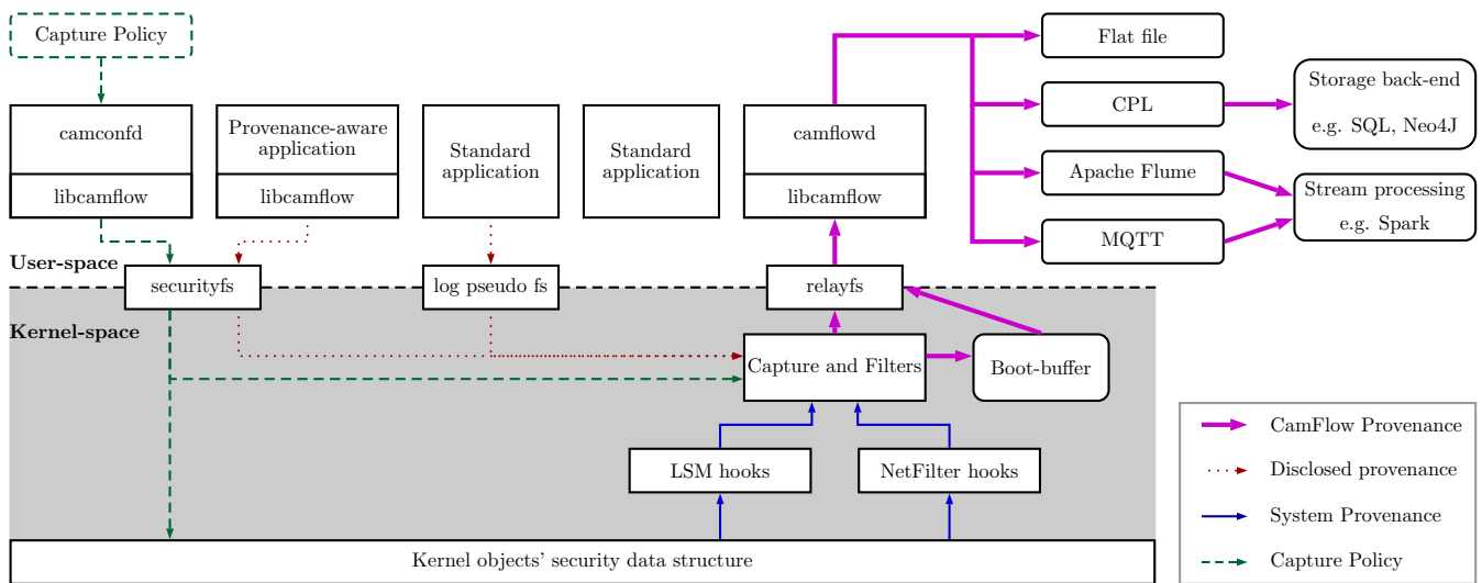
Figure 4: Architecture overview.
