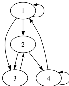
Figure 1: A Markov Chain with 4 Recurrent States
