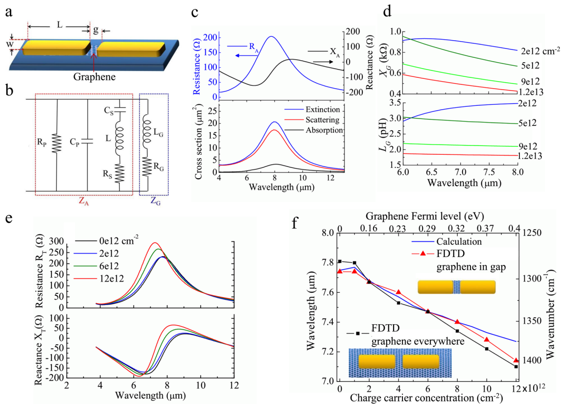
Figure 2. Circuit model for graphene loaded antenna pair. (a) Schematic of an antenna pair, loaded with a graphene sheet in the gap ( g = 20 nm, L = 1.84 \mu\text{m} , w = 240 nm). (b) Effective circuit model of the structure in (a). Z_A is the antenna impedance and its effective circuit elements are R_p = 1.0 k \Omega , C_p = 3.21\text{E}-17 F, C_s = 3.84\text{E}-17 F, L = 9.2\text{E}-13 H, R_s = 63 \Omega . Z_G is the graphene load impedance; L_G and R_G represent its inductance and resistance, respectively. (c) Input resistance and reactance (real part and imaginary part of the impedance Z_A ) of the antenna in part a, and extinction, scattering, and absorption cross sections extracted from FDTD simulations. (d) Reactance ( X_G ) and inductance ( L_G ) of the graphene load in antenna nanogap ( g = 20 nm, w = 240 nm). (e) Resistance and reactance (real part and imaginary part of the impedance Z_T ) of the graphene loaded dipole antenna for different carrier concentrations. (f) Scattering resonance peaks obtained from the circuit model (solid line: calculation), FDTD simulation (stars: antenna pair with graphene only in the gap; squares: antenna pair on a large graphene sheet) as a function of graphene carrier concentration. The corresponding graphene Fermi levels are given on the top axis beside the major ticks.
