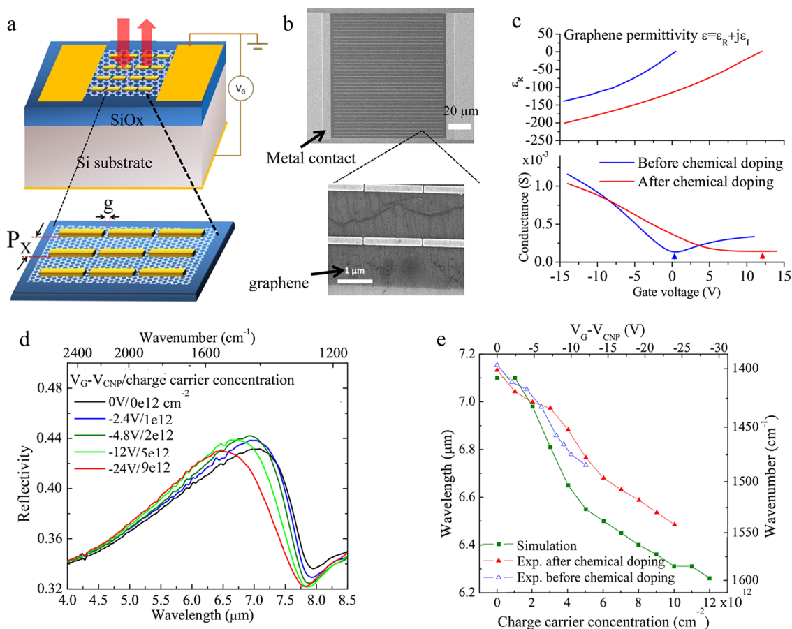
Figure 4. Device configuration and experimental results of antenna array with tunable resonance. (a) Schematic of the tunable plasmonic device with back gate voltage and the antenna array on a gated graphene sheet. (b) Scanning electron microscope (SEM) image of one device and a zoomed-in portion of the antenna array on graphene. (c) Measured graphene conductance (bottom) and calculated graphene permittivity (top) for graphene samples before and after chemical doping as a function of gate voltage. (d) Measured reflection spectra from an antenna array after chemical doping (antenna length 1.8 \mu\text{m} , gap size 20 nm, lateral period 2.6 \mu\text{m} ) for different gate voltages V_G ( V_{\text{CNP}} is the gate voltage at the charge neutral point, where the numbers of holes and electrons in the graphene sheet are equal.) and the corresponding charge carrier concentrations. (e) Simulated (solid red squares) and measured (blue open triangles: before chemical doping, red solid triangles: after chemical doping) reflectance peak wavelengths for the same antenna array as a function of gate voltage and charge carrier concentration.
