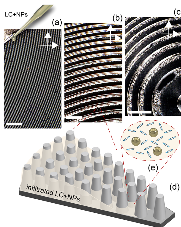
Figure 2. Polarized optical microscopy (with the metalens between crossed polarizers ( 90^\circ ), shown as perpendicular arrows) image of 6CB+AuNPs filled metalens along the (a) far edge, (b) inner, and (c) central region; scale bar: 200 \mu\text{m} . The pipet in (a) illustrates a droplet of LC placed at the edge of the lens during the infiltration procedure. (d) Illustration of a pillars region of the metalens infiltrated with the 6CB+AuNPs mixture (e).
