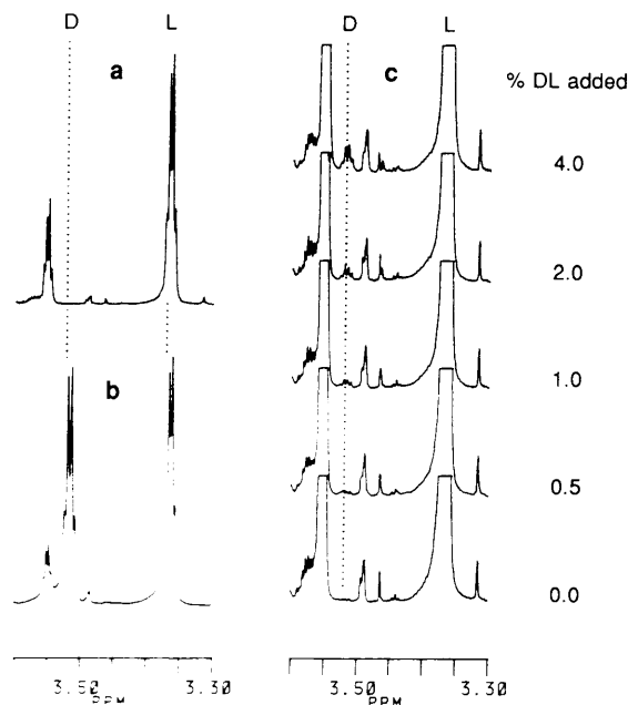
Figure 9. ^1\text{H} NMR spectra (300 MHz) at 3.30–3.60 ppm of the methoxy ether peaks of the ( R )-(+)-MTPA derivatives of (a) methyl L - \alpha - cis -crotylglycinate, (b) methyl DL - \alpha - cis -crotylglycinate, and (c) a + 0.0–4.0% of b (base-line detail).
