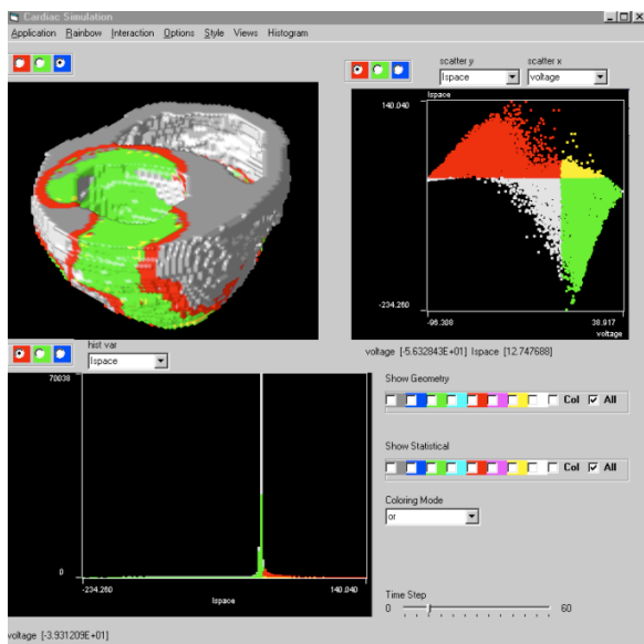
Fig. 5 Screen Shot of “WEAVE” in action. Colored selections can be made in any of the 2D analysis panels, or directly in the high-dimensional (3D) display, and all views are live-linked. From Gresh et al. (2000).
