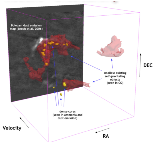
Fig. 8 “Astronomical Medicine” view of L1448, created using 3D Slicer by Jens Kauffmann. Similar figures were published as the first interactive 3D PDFs in the journal Nature (Goodman et al. 2009).
