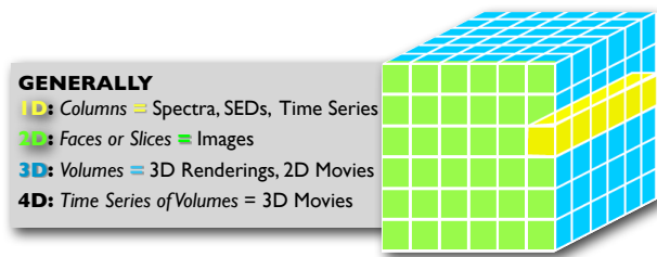
Fig. 2 Data “Cubes” in Astronomy.
